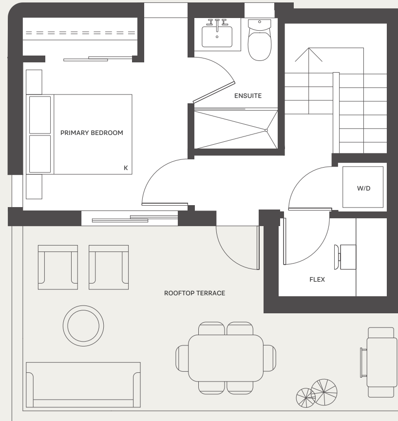
SECOND LEVEL
