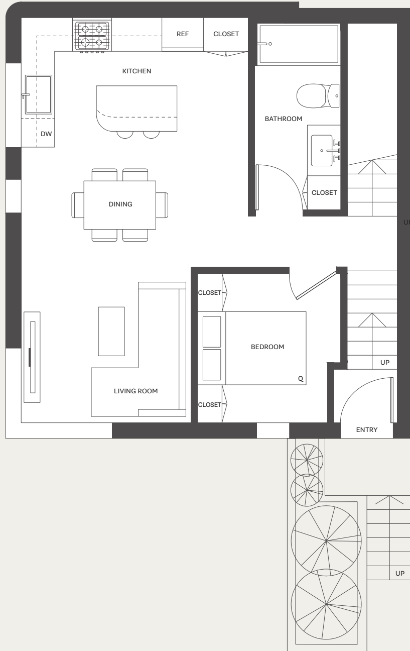
MAIN LEVEL
