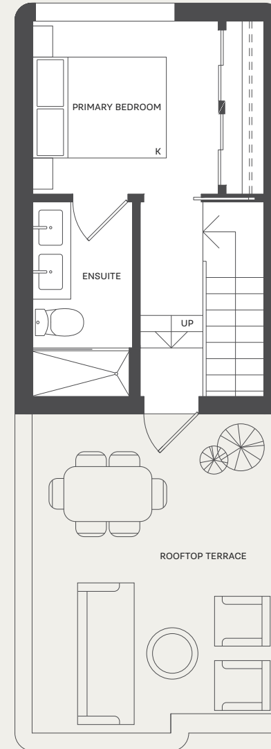
THIRD LEVEL
